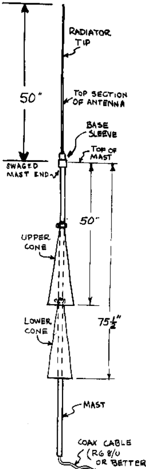
ASSEMBLY DRAWING
